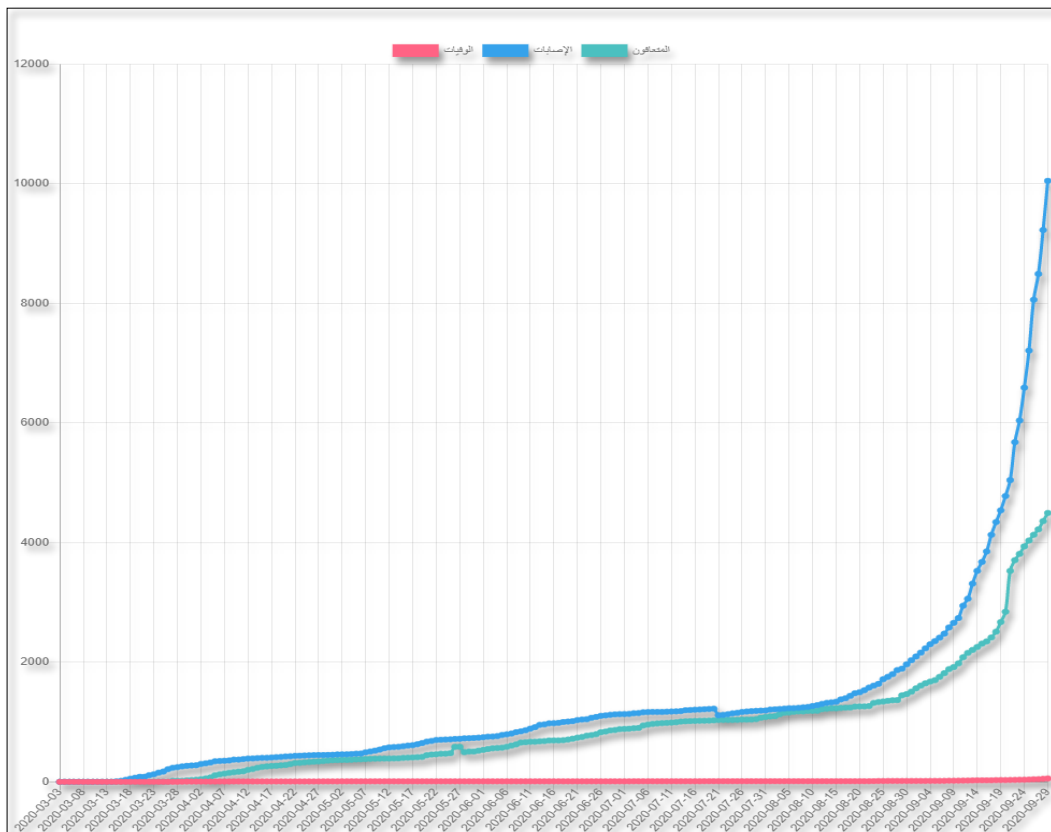
Figure 2. Statistics of the spread of Corona virus in Jordan.
