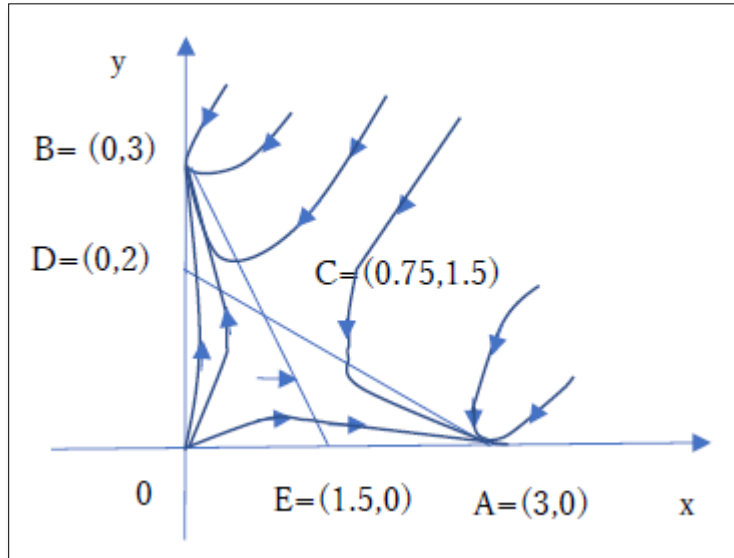
Figure 2. Sketch of the track for the roots.
