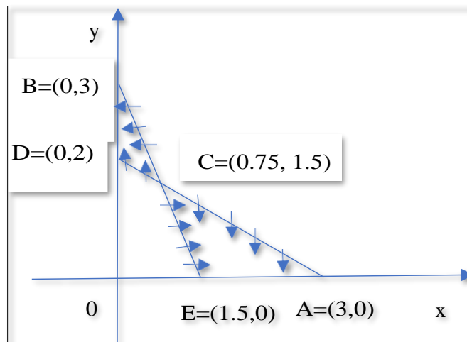
Figure 1. Two lines on which dy/dx=0 or \pm\infty .
