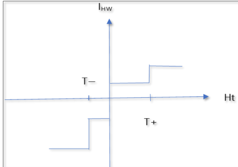
Figure 3. I_{HW} against H_t . T_+ is the positive threshold; T_- is the negative threshold.
