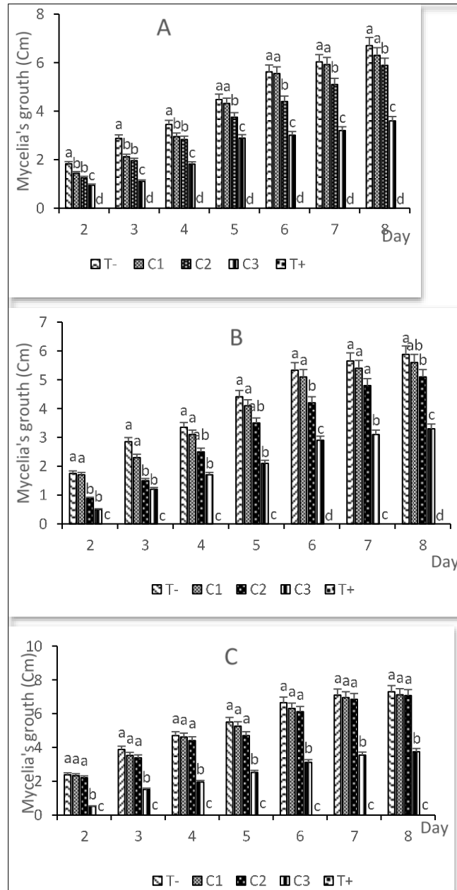
Figure 3. Effects of HEC on different strains of S. sclerotiorum at different concentrations: A- Bia 1, B- Bia 2, C-Njo 2. *Values for the same day with different letters are significantly different at p < 0.05 (LSD test)
