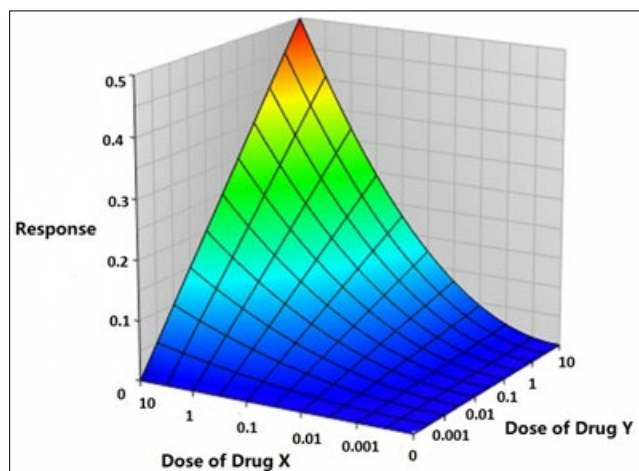
Figure 2. Example of response surface for two drugs, X and Y. The doses of individual drugs are plotted as a horizontal x-y-plane, and the expected effect (response) of drug combination is plotted on the z-axis.
