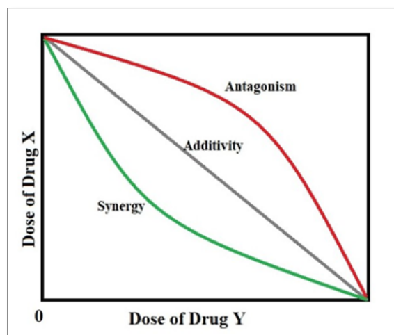
Figure 1. Comparison of additive, synergy and antagonism at the same response level. If the drug combination X and Y achieves the same response level with less dose than that of additive case (the reference model), the combination is said to be synergistic.
