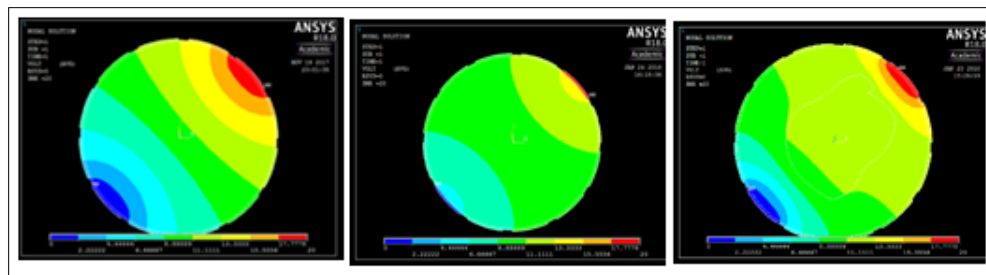
Figure 9. Voltage distributions for air, water and bone in ECT sensor.
