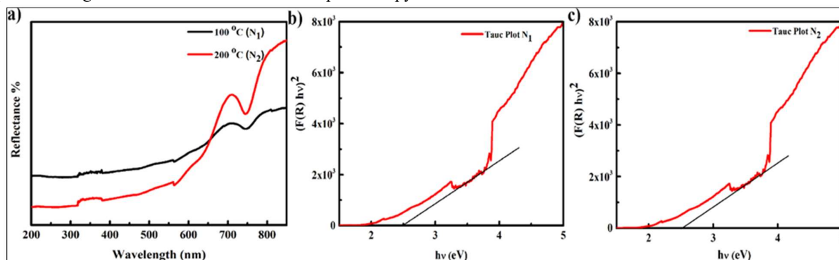
Figure 7. UV- Vis DRS spectra of a) \text{NiFe}_2\text{O}_4 at 100^\circ\text{C} ( \text{N}_1 ) and \text{NiFe}_2\text{O}_4 at 200^\circ\text{C} ( \text{N}_2 ). b) and c) Tauc Plot for \text{N}_1 and \text{N}_2 .
