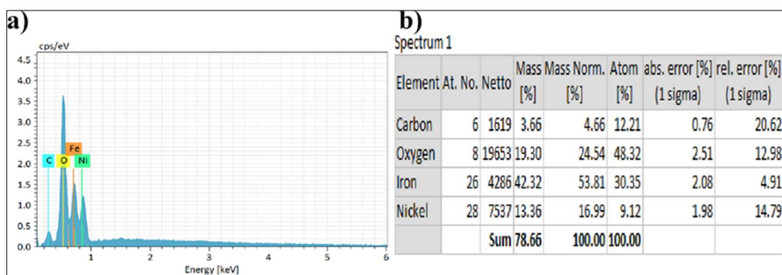
Figure 5. a) the EDAX spectrum and b) is the table showing the atomic weight percentage of each element in the \text{NiFe}_2\text{O}_4 at 200^\circ\text{C} ( \text{N}_2 ) sample.
