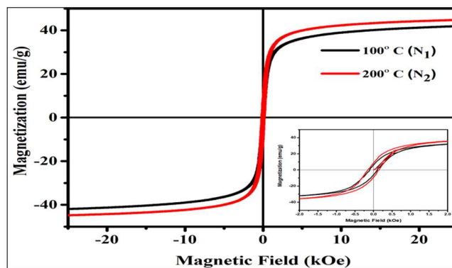
Figure 6. The M-H hysteresis loop showing the variation of magnetization value with applied magnetic field for the synthesized \text{NiFe}_2\text{O}_4 at 100^\circ\text{C} ( \text{N}_1 ) and \text{NiFe}_2\text{O}_4 at 200^\circ\text{C} ( \text{N}_2 ).
