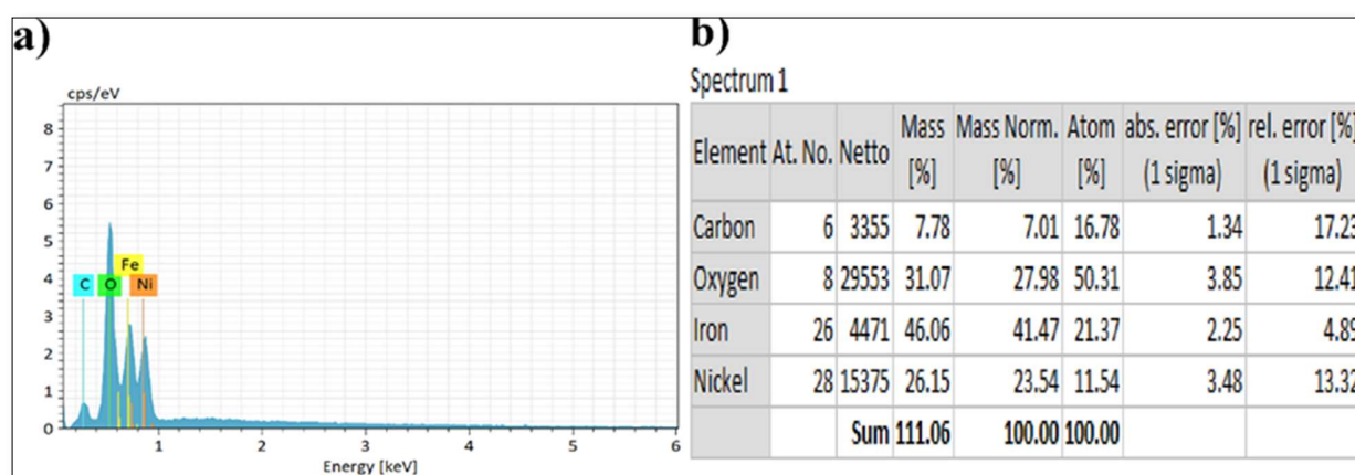
Figure 3. a) the EDAX spectrum and b) is the table showing the atomic weight percentage of each element in the \text{NiFe}_2\text{O}_4 at 100^\circ\text{C} ( \text{N}_1 ) sample.
