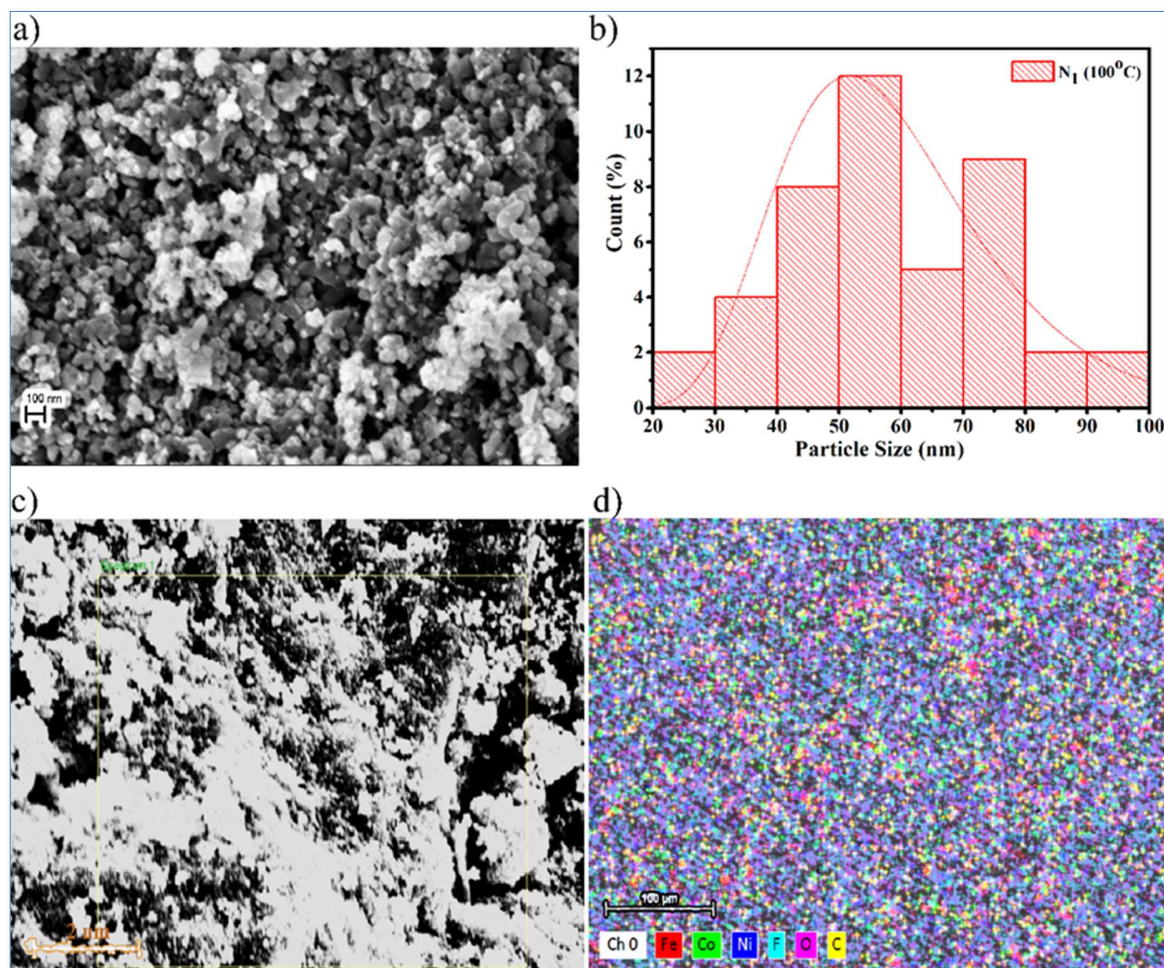
Figure 2. a) and b) represents the FESEM micrograph and histogram of particle distribution c) and d) corresponds to the EDAX image mapping for \text{NiFe}_2\text{O}_4 at 100^\circ\text{C} ( \text{N}_1 ).
