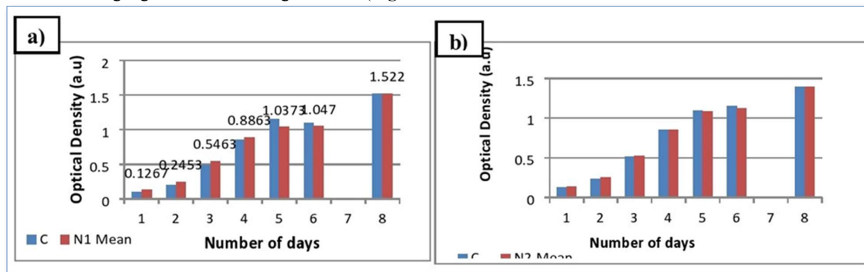
Figure 8. a) and b) represents the variation of Chlorophyll-a growth for a time gap of 48h for the control (without nanoparticles) and NiFe 2 O 4 calcined at two temperatures.
