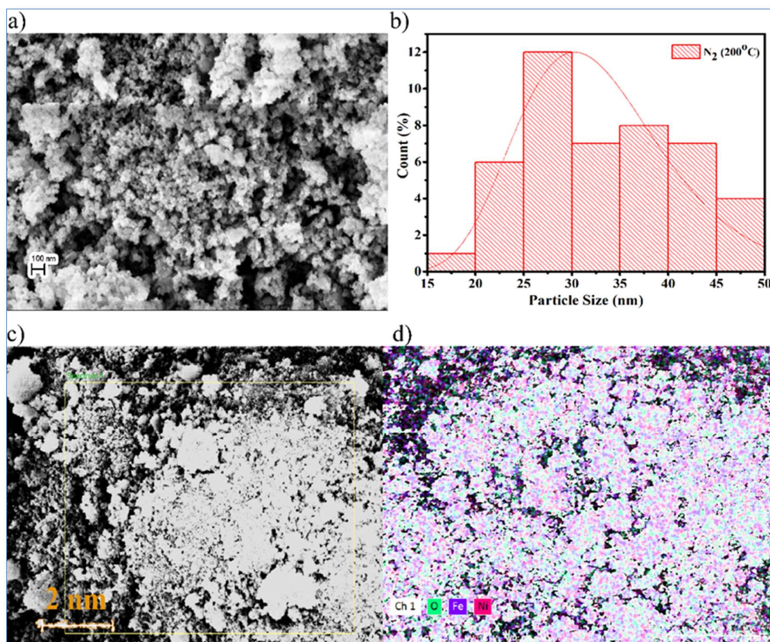
Figure 4. a) and b) represents the FESEM micrograph and histogram of particle distribution c) and d) corresponds to the EDAX image mapping for \text{NiFe}_2\text{O}_4 at 200^\circ\text{C} ( \text{N}_2 ).
