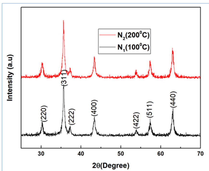
Figure 1. XRD diffractogram for \text{NiFe}_2\text{O}_4 at 100°C ( N_1 ) and \text{NiFe}_2\text{O}_4 at 200°C ( N_2 ).
