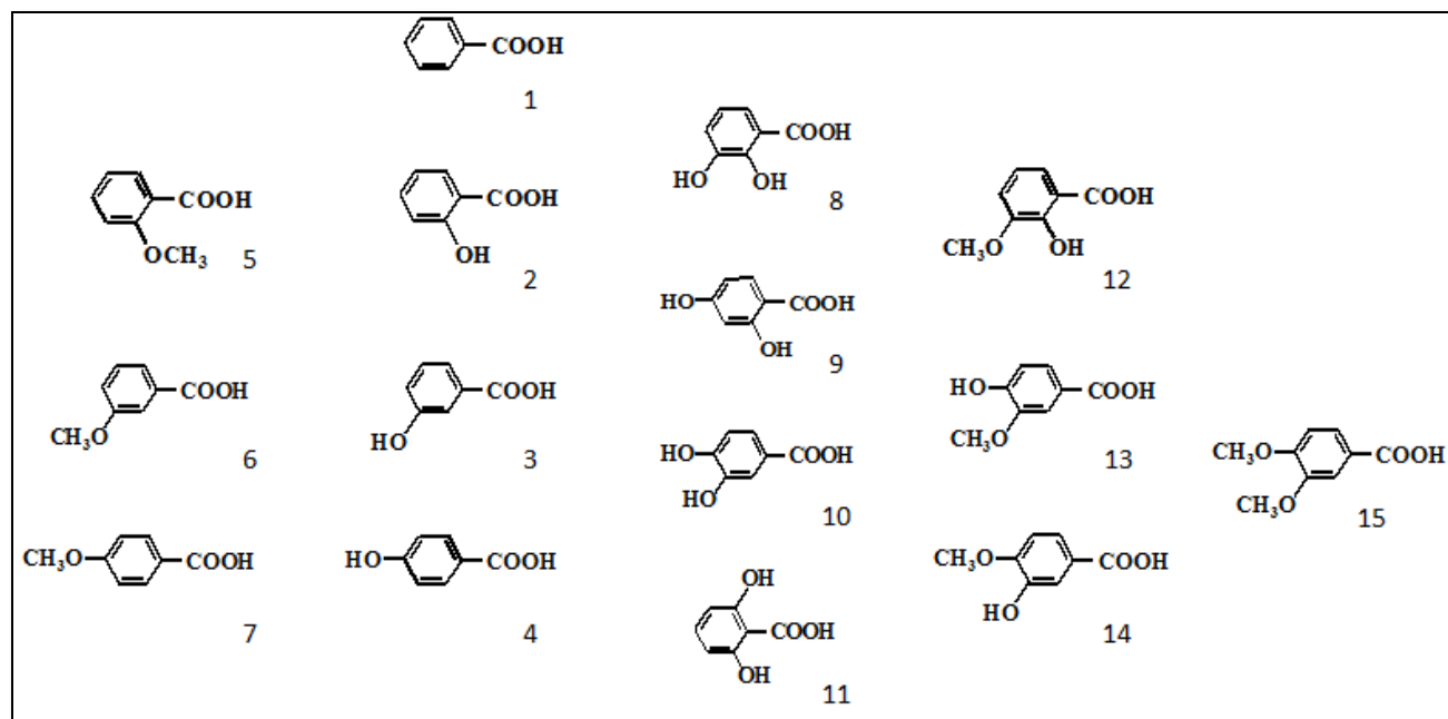
Figure 1. Structures of benzoic acid derivatives.
