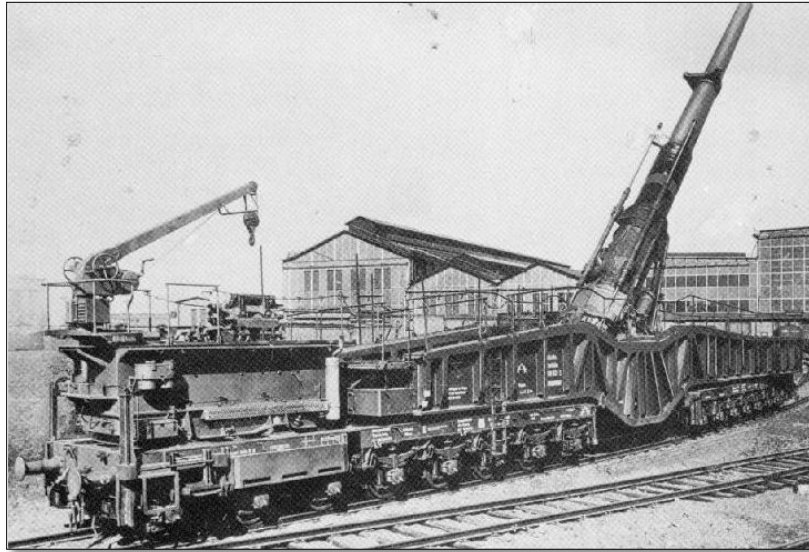
Figure 2. 'Lange Max', a 'Lange Ludwig' prototype from 1912.
