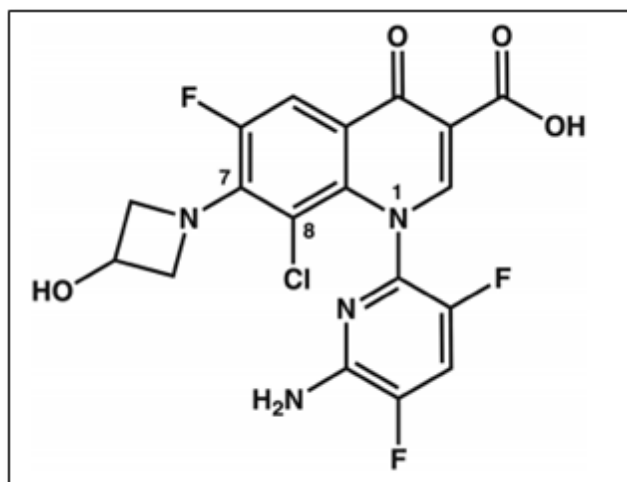
Figure 1. Chemical structure of delafloxacin ( C_{18}H_{12}ClF_3N_4O_4 ).
