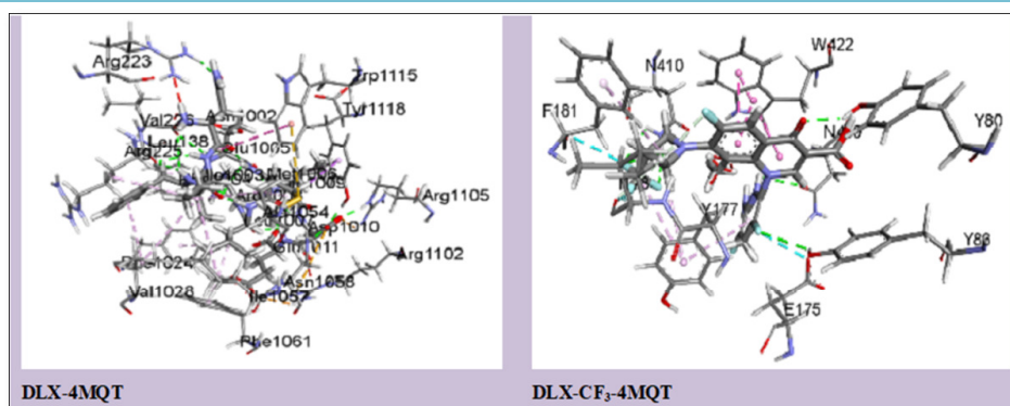
Figure 4. Binding sites of ligands-proteins.
