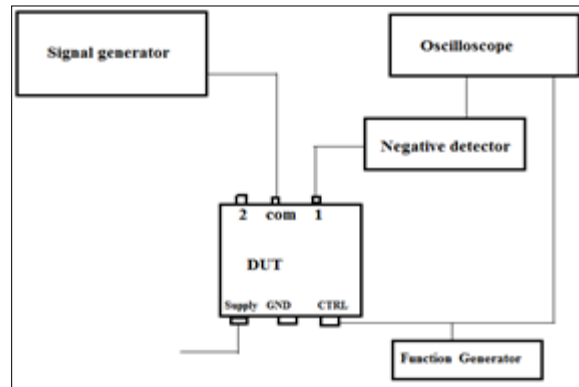
Figure 7. Test unit for switching time measurement.
