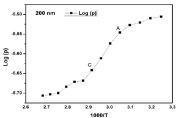
Figure 5. Graph between Log ( \rho ) and 1000/T for 200 nm Zn/Te thin films.
