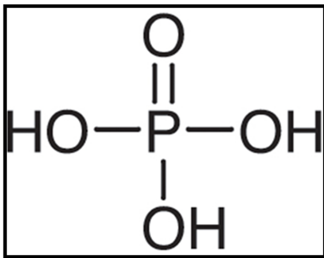
Figure 1. Chemical structure of Phosphoric acid.
