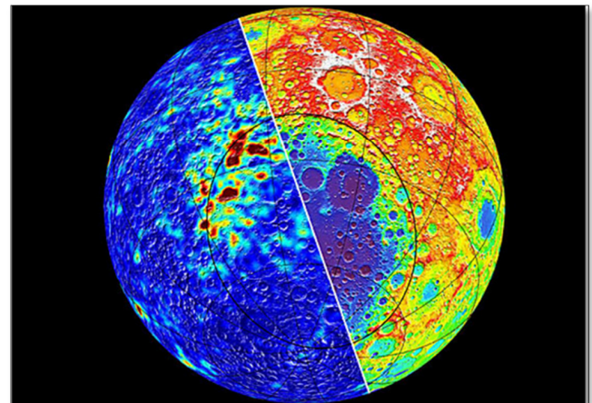
Figure 3. The Moon's magnetic rocks are pictured to the left in dark red.
