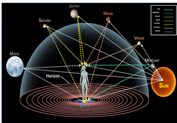
Figure 2. Sunlight on the Earth directly, by Reflection, by Deflection and Reflection, and by Modulation through the Lunar Nodes.
