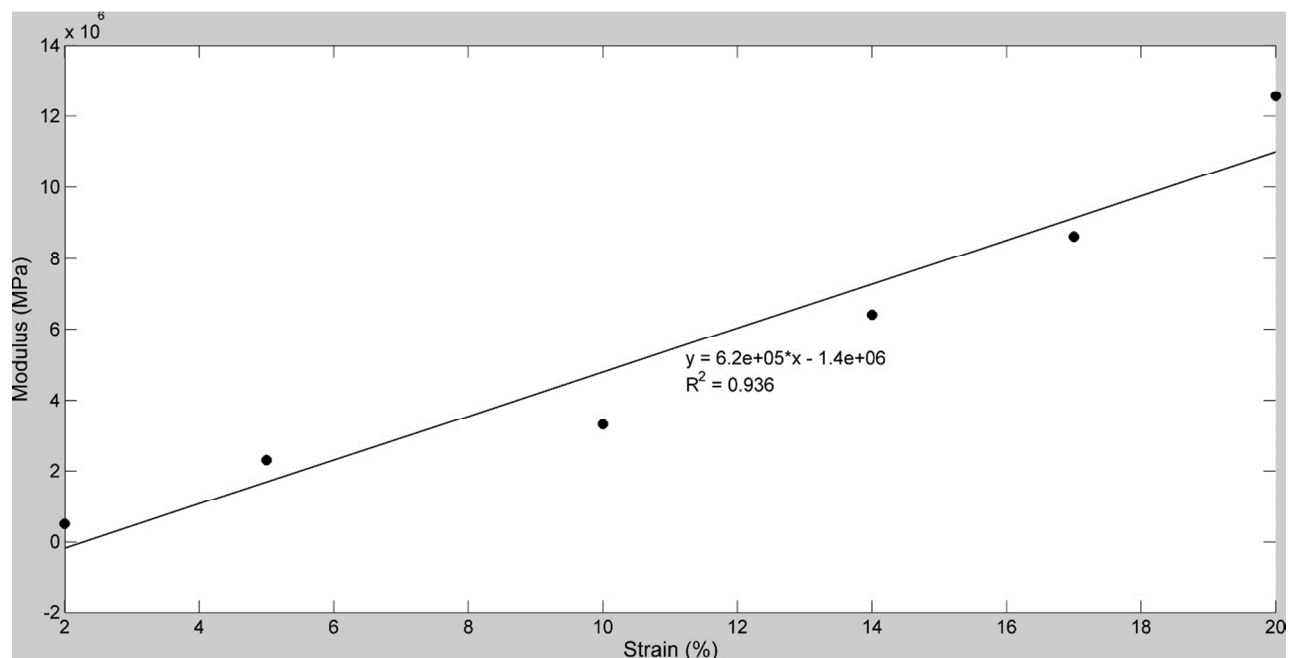
Figure 3. Plot of modulus determined from OCT and vibrational studies versus strain for decellularized dermis. Note the resonant frequency and modulus increases with strain due to the increased recruitment of collagen fibers with increasing strain during stretching.
