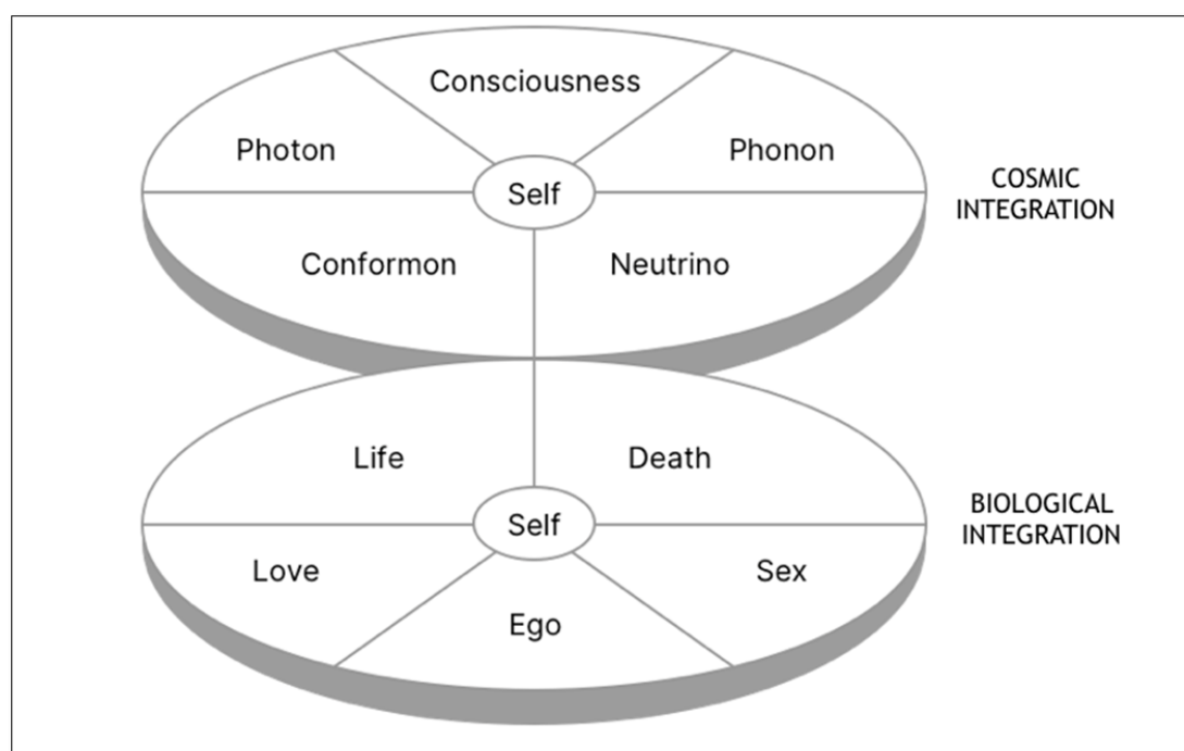
Figure 5. Cosmic Integration machinery, self with phenomenal hands of Mother Nature, interacts with the biologically integrated brain accommodating consciousness's CEO inside the system, the self, which has achieved the phenomenological integration. The footprints of elementary phenomena which were involved during genesis of self from consciousness surround this self, as its private facets.
