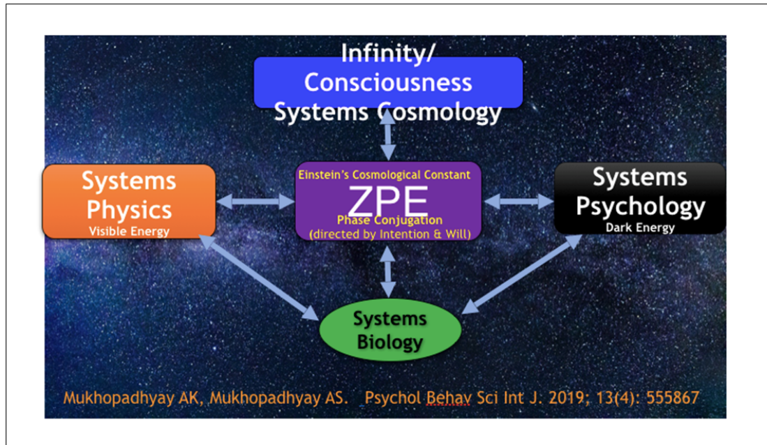
Figure 6. ZPE is the point of meeting, coupling, conjugation and fertilization of systems physics, systems psychology, systems biology and systems cosmology. Systems Physics are driven by visible energy. Systems psychology is mostly driven by dark energy. Visible and dark energy are balanced by systems biology. The verticality in the process seems obvious since the coupling, conjugation and fertilization are driven not by any force or energy but by intention and will which come from consciousness at the vertical depth of nature (Infinity).
