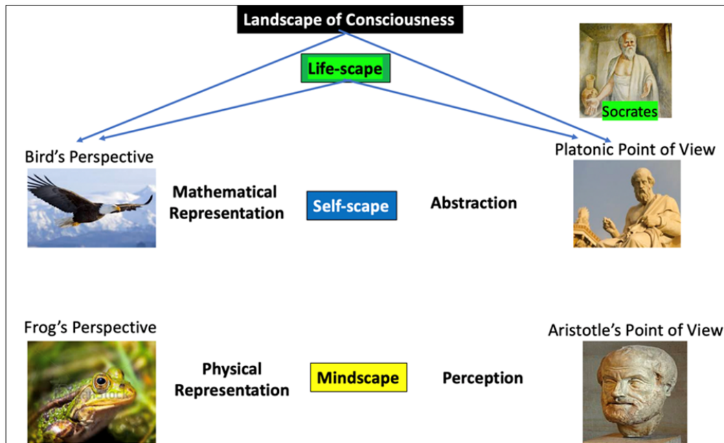
Figure 9. The behavioral description of the Multiverse depends on the cognitive faculty of the scientists; his mindscape, self-scape, life-scape and finally the consciousness-scape. Physical perception is from Aristotelian point of view and is often called frog's perspective. This is a picture in the mindscape of the scientist. Mathematical abstraction is from Platonic point of view and is often called bird's perspective. This is the picture in the self-scape of the scientist. Life-scape covers both mindscape and self-scape. The landscape of consciousness overarches life-scape, self-scape and mindscape.
