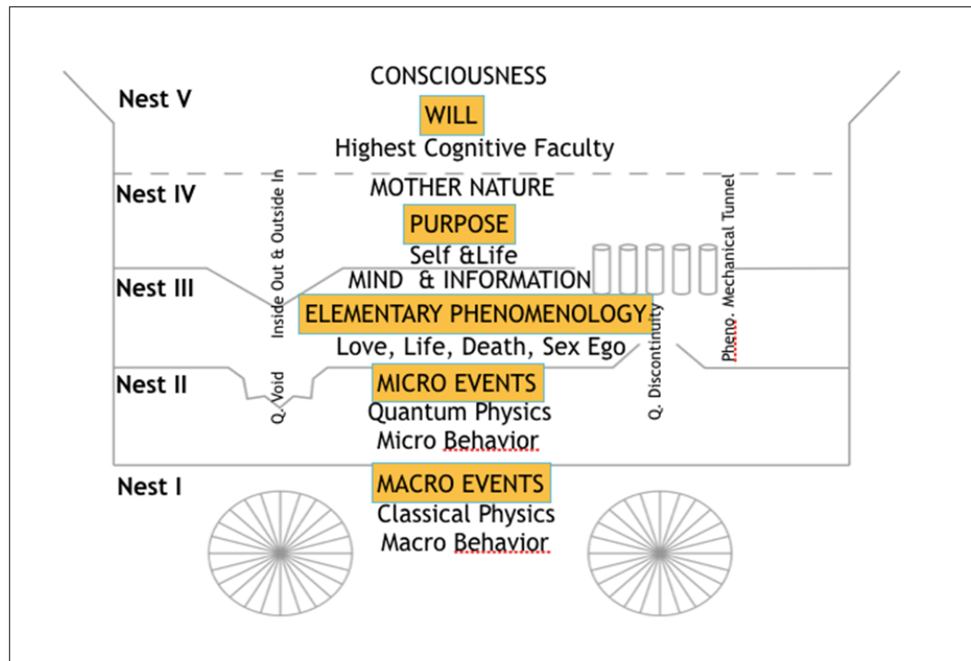
Figure 4. Five nests of Nature-Consciousness (Five-in-One, Pentaune Model). Nest I is the domain of classical physics and Nest II is of quantum physics. Nest III is the domain of mind, information, intelligence and emotion. Nest IV is the domain of Mother Nature and Nest V is that of Consciousness. Nest V is the nest of Will. In Nest IV the purpose is determined. Nest III is the nest for elementary phenomenology to achieve the purpose. Nest II has a number of micro-events from the phenomenology and Nest I is full of corresponding macro-events observable to all.
