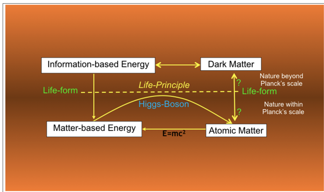
Figure 11. Life-form stands at the boundary of Nature within Planck's scale and Nature outside Planck's scale. Information-based energy is converted to visible energy by life-form. We are not aware of the mechanism of interconversion of dark matter and atomic matter and whether life-form has any role in this mechanism.
