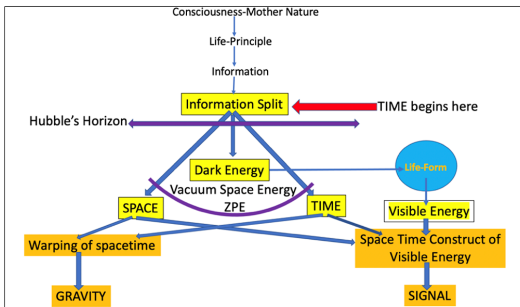
Figure 10. Consciousness-Mother Nature is the ultimate Source field. Life-principle is the source field of information. Splitting of information is the beginning of Time. Space Time and Dark energy are three children of information. Warping of space time creates gravity. Conversion of dark energy into visible energy requires life-form. Visible energy in unit of space per cycle of time constitutes signal.
