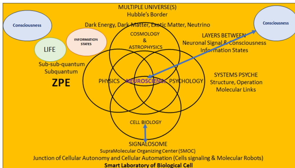
Figure 12. In this self-explanatory figure, intersections of several disciplines of science have been shown. Neuroscience is at the centre of intersections. Zero-Point Energy (ZPE) is in focus. So also, is “life”. Multiple universe (s) are at the top and the smart cellular laboratory is on the ground. The Top connects with the Bottom through several disciplines of science.
