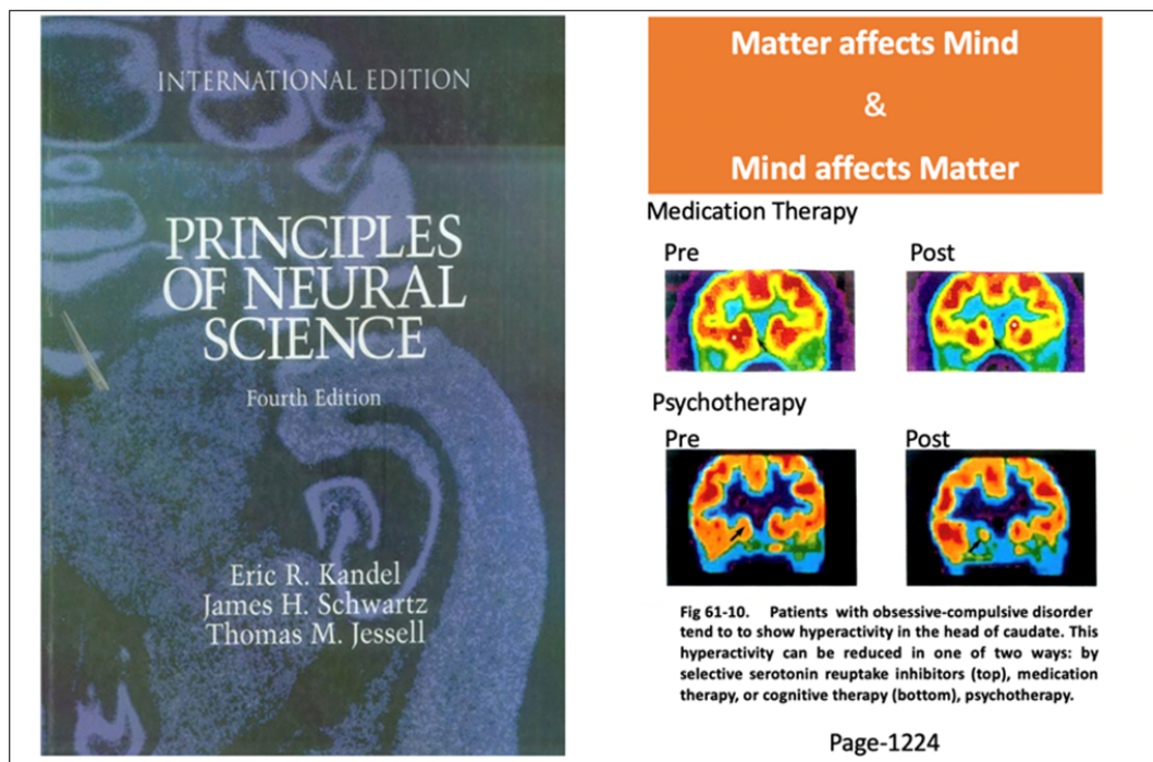
Figure 8. A patient of OCD shows significant hyperactivity at the head of caudate nucleus. This could be brought to near normal by both medication and psychotherapy. This shows Mind affects Matter and the Matter affects Mind. The neuroimage shown in the right side of the figure has been taken from old International Edition of the text book of Principles of Neural Sciences, page 1224. In later edition of the book, this important picture is missing. The caption of the heading on the image is modified by the author.
