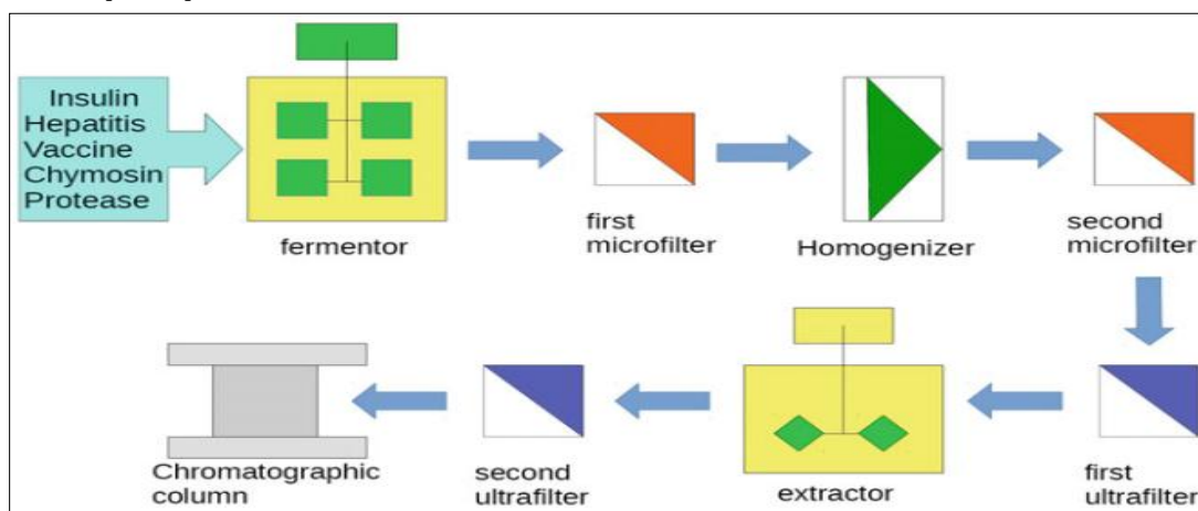
Figure 1. Multiproduct batch plant for protein production.
