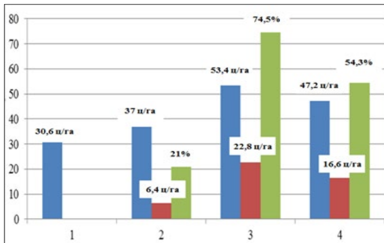
Figure 3. The effect of minimum processing and fertilizer rates on the yield of winter wheat (for 3 years). E=0.75-1.06 t/ha; P=1.83-2.50\%
