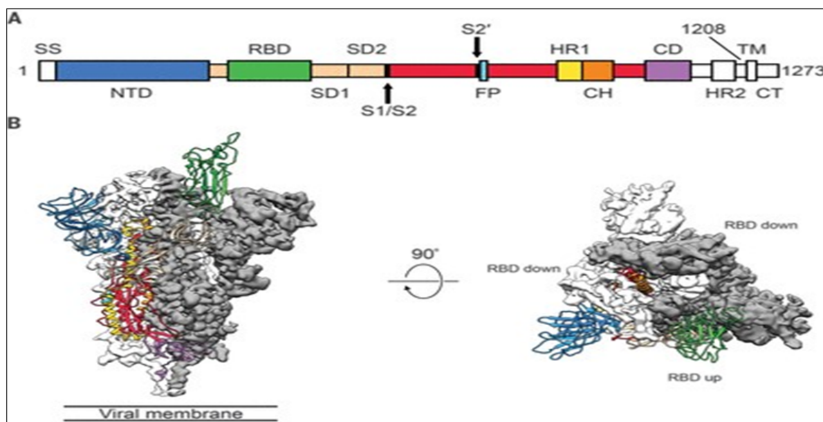
Figure 1. Structure of 2019-nCoV S in the pre-fusion conformation [1].
