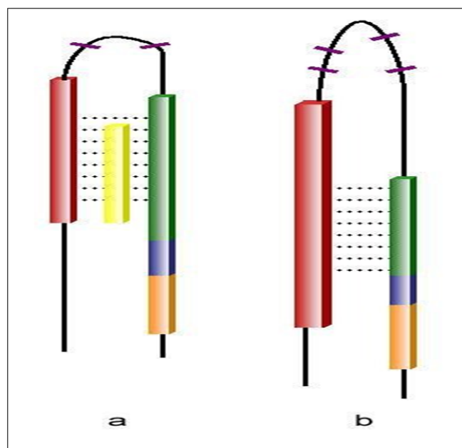
Figure 2. Similarity between the fusion proteins of HIV-1 and SARS-CoV. The HIV-1 gp41 (a) and the equivalent S2 protein from the SARS-CoV (b) are shown. A Leucine/Isoleucine heptad repeat adjacent to the N-terminus of both proteins appears in red. The C-terminal heptad repeat is in green. Cysteine residues (purple) confining a loop structure is located between the two heptad repeats. An aromatic residues-rich motif is marked blue, and the transmembrane segment is in orange. A peptide corresponding to the C-terminal heptad repeat, which acts as potent inhibitor of HIV-1 entry into the cell, appears in yellow [5].
